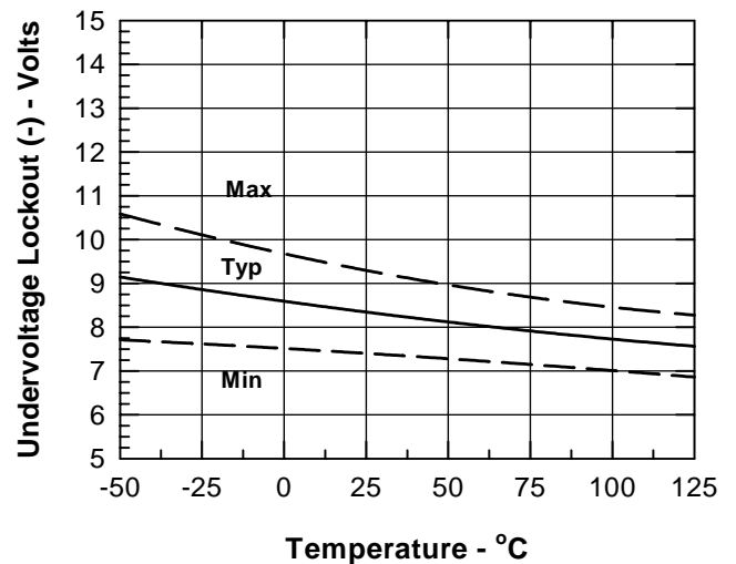
Fig. 24b. V_{CL} Undervoltage negative trip vs. temperature.
